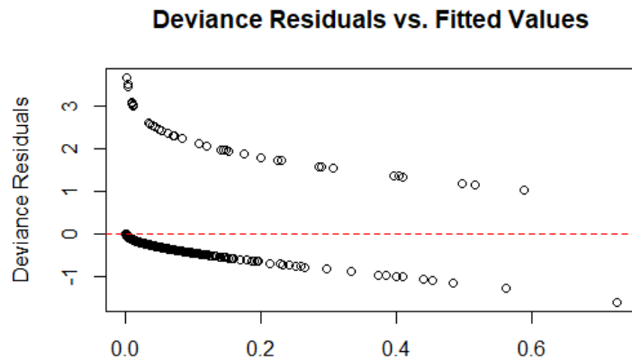
Fig. 7. Deviance plot
